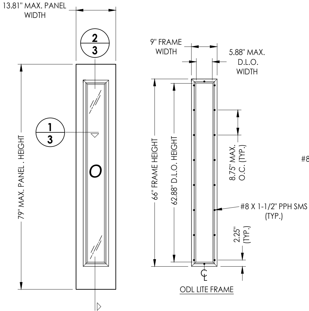
50 STEEL SIDELITE PANEL ODL, INC.
